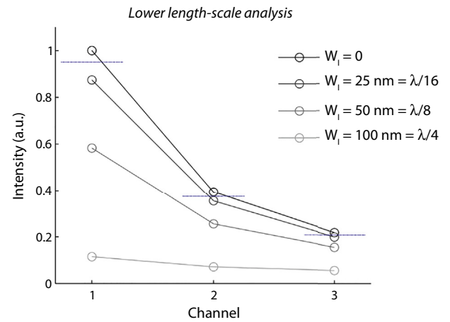
Supplementary Figure 2. Probing the lower length-scale sensitivity of the spatially resolved subdiffuse reflectance spectroscopy (SRSRS) probe using Monte Carlo (MC) simulations. A continuous random media representing tissue 22 was simulated using MC. A gaussian filter was used to remove small structures below a specific size, using the method previously described by Radosevich et al. 25 Each media with a size of structures removed was simulated with MC and compared with the unmodified media. A measured change greater than 5% for each of the 3 probe channels was considered significant enough to measure in practice. The results show that removal of structures as small as 25 nm result in >5% change in measured scattering by the SRSRS probe.
